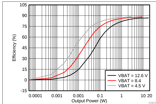
Figure 6. Efficiency vs Output Power
