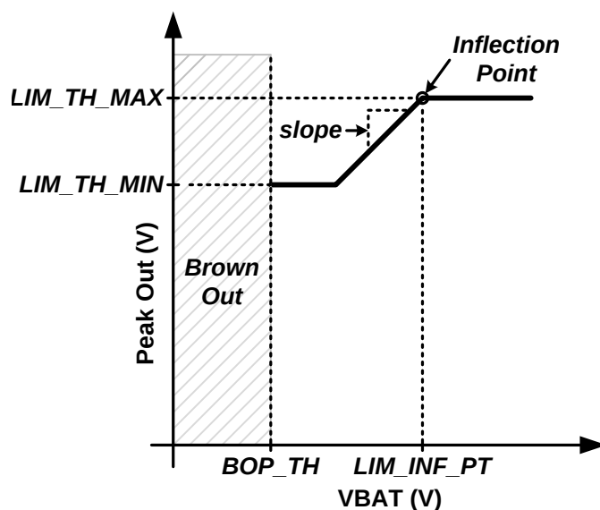
Figure 25. Limiter with Inflection Point and Minimum Threshold
