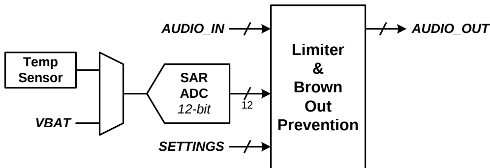
Figure 26. Limiter Block Diagram
