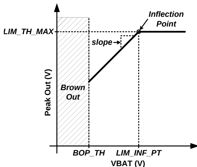
Figure 24. Limiter with Inflection Point
