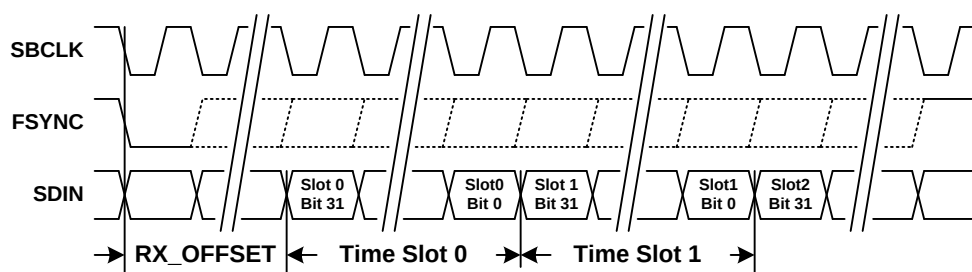
Figure 20. TDM RX Time Slots
