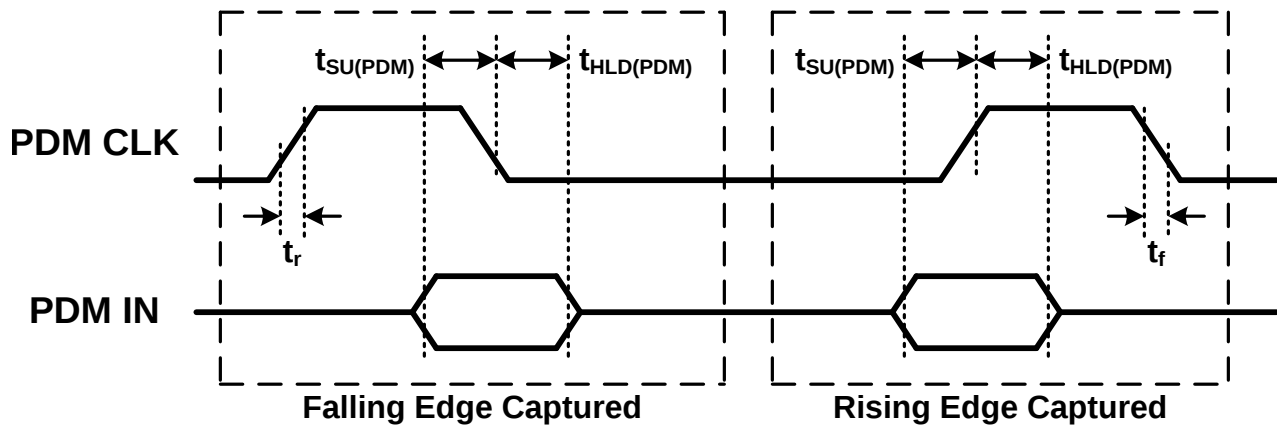
Figure 4. PDM Timing Diagram
