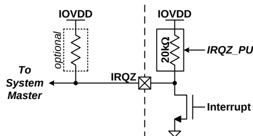
Figure 29. IRQZ Pin
