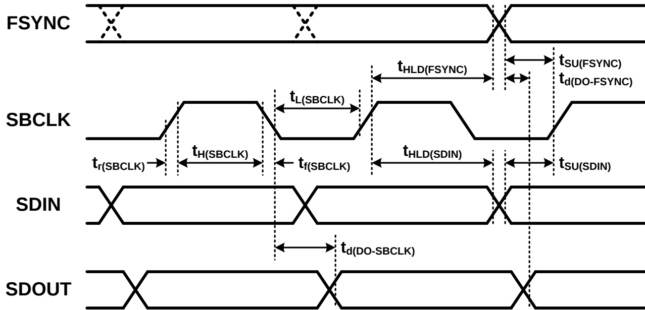
Figure 3. TDM Timing Diagram
