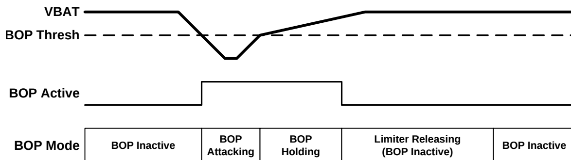
Figure 27. Brown Out Prevention Event
