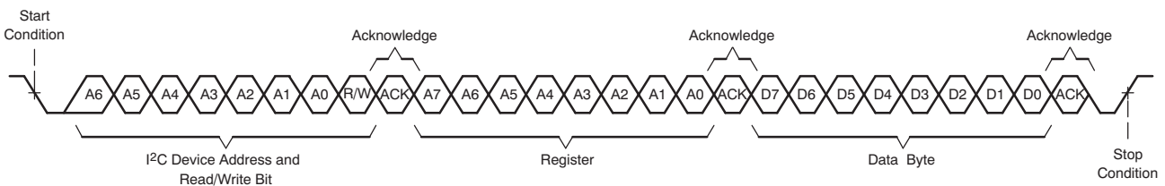
Figure 13. Single-Byte Write Transfer
