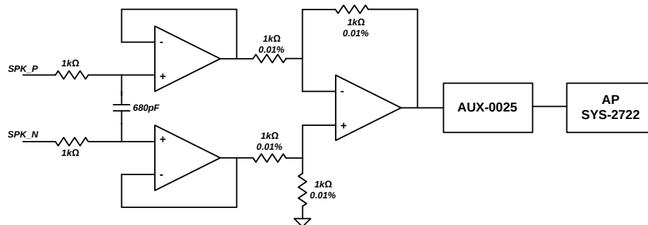
Figure 11. Differential To Single Ended (D2S) Filter
