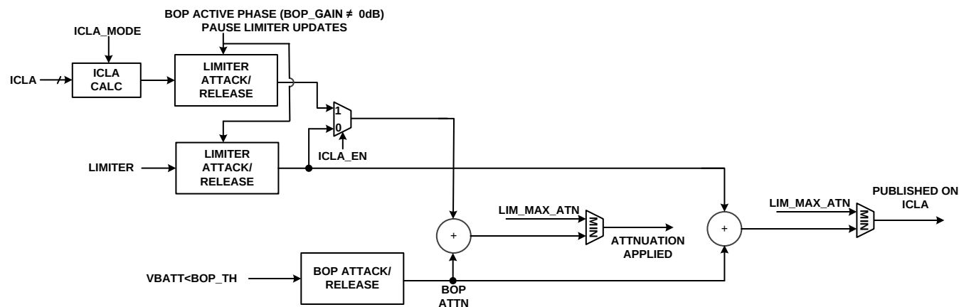
Figure 22. Limiter and Brown Out Prevention Interaction Diagram
