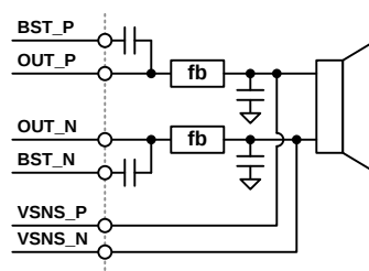
Figure 28. V-Sense Connections
