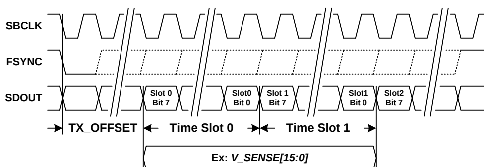
Figure 21. TDM Port TX Diagram
