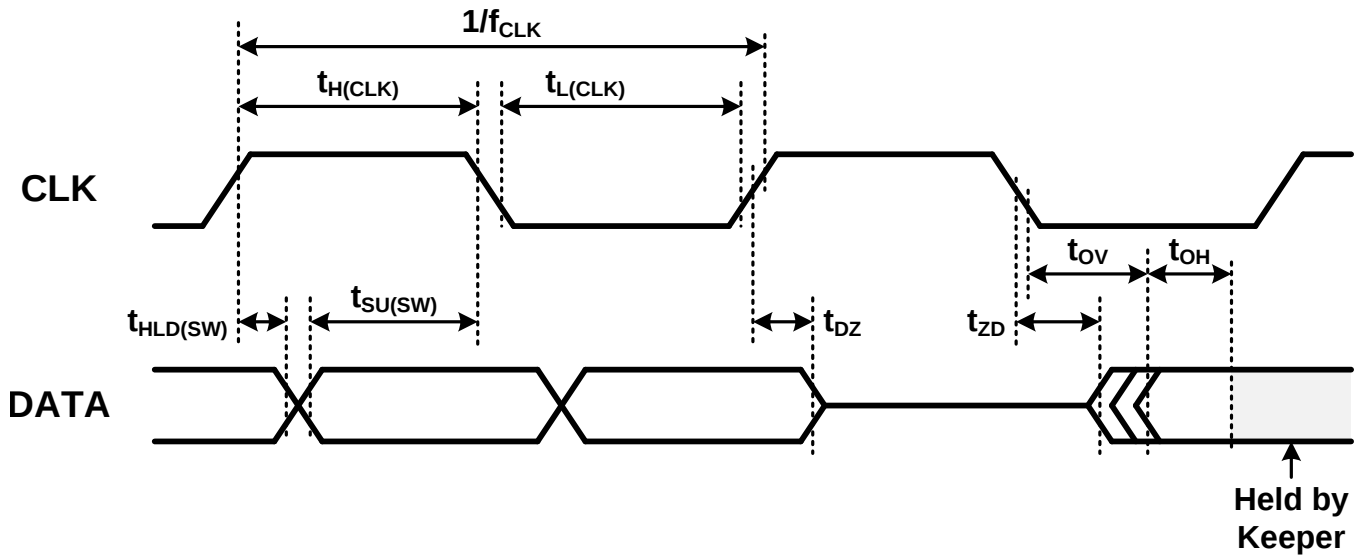
Figure 5. Soundwire Timing Diagram
