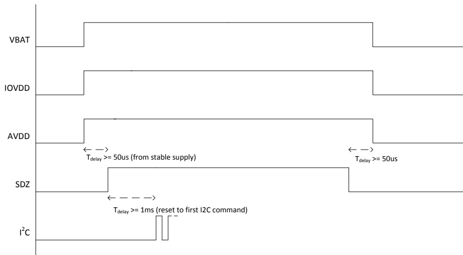
Figure 83. Power Supply Sequence for Power-Up and Power-Down
