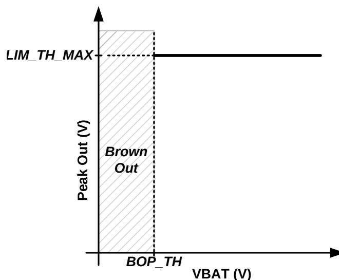
Figure 23. Limiter with Fixed Threshold
