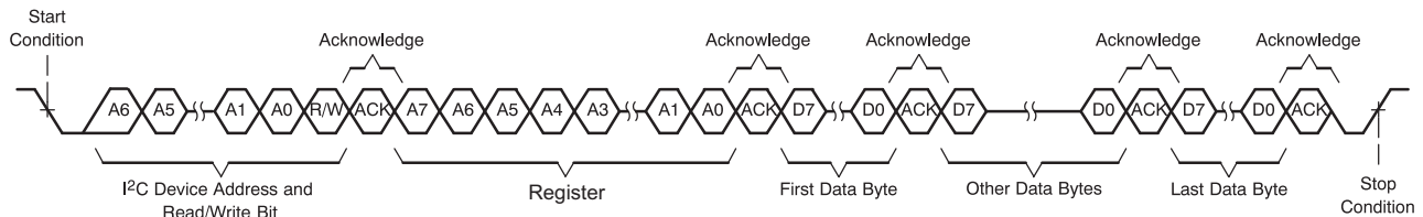
Figure 14. Multi-Byte Write Transfer
