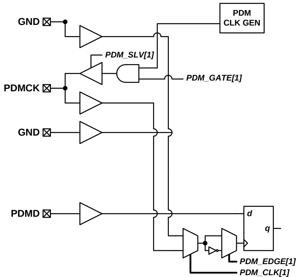
Figure 18. PDM Data and Clock Input Block Diagram
