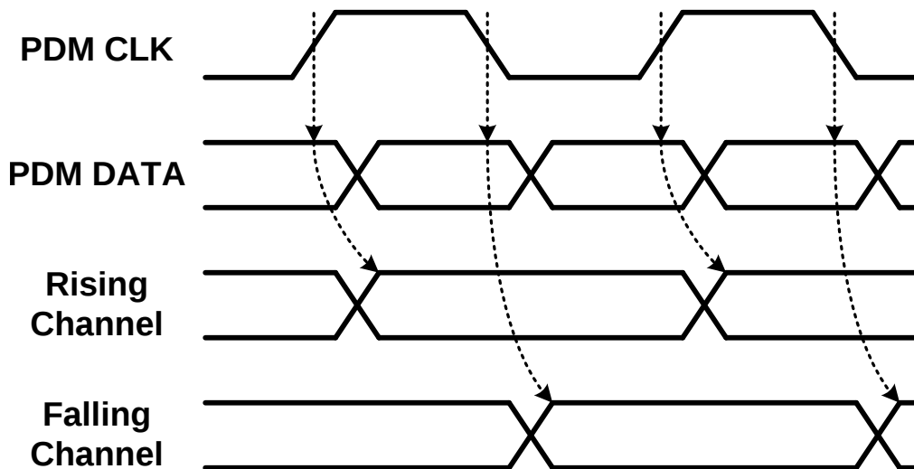
Figure 17. PDM Waveform
