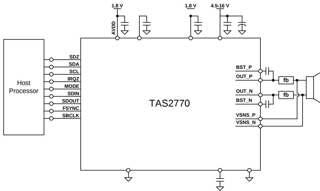
Figure 80. TAS2770 Typical Application
