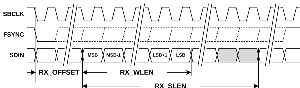
Figure 19. TDM RX Time Slot with Left Justification
